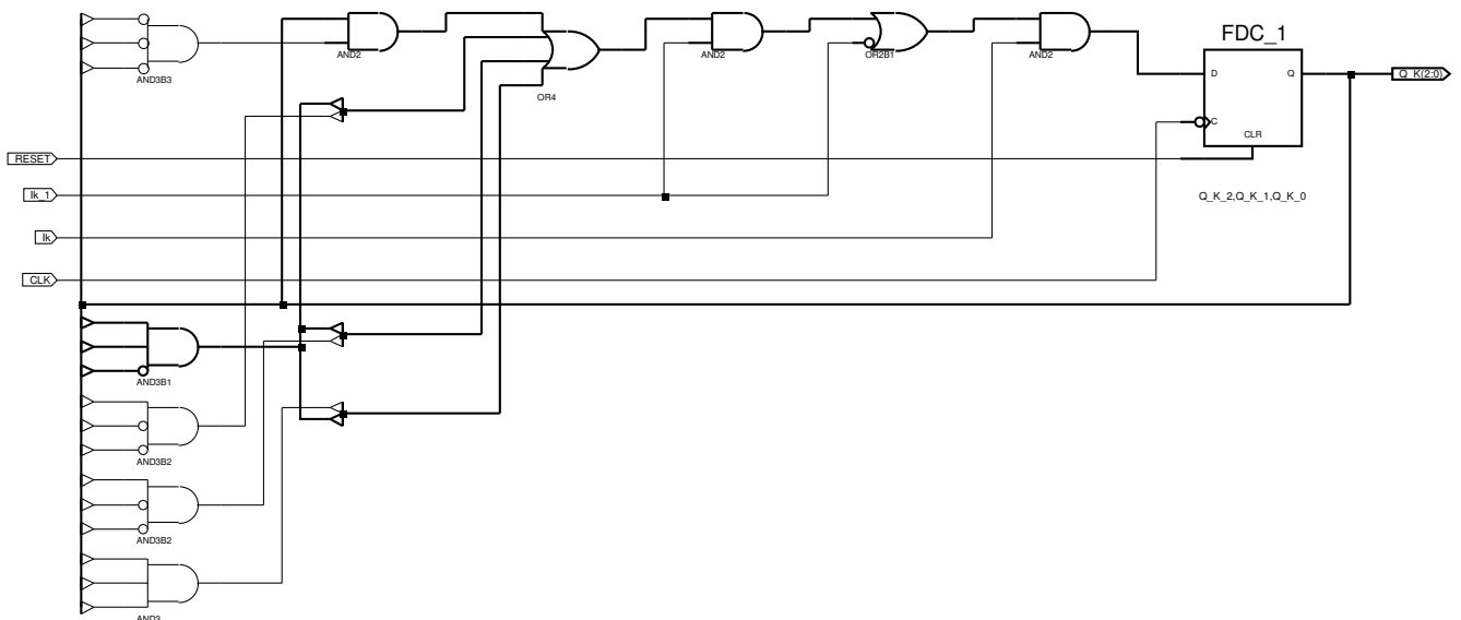
Figure 4. AC module automata for band 7.
