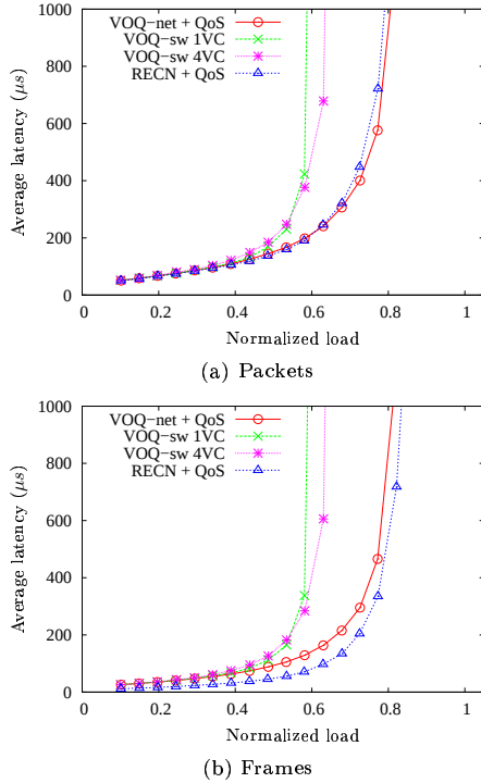
Figure 4: Performance in video transmission scenario.
