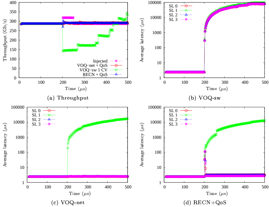
Figure 3: Results for hot-spot scenario.
