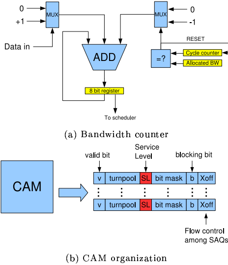
Figure 2: CAMs and bandwidth counters.
