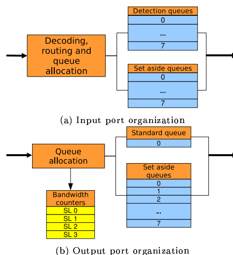
Figure 1: Input and output ports logical organization.
