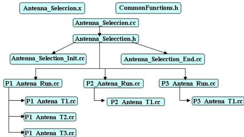
Fig. 7. Generated files
